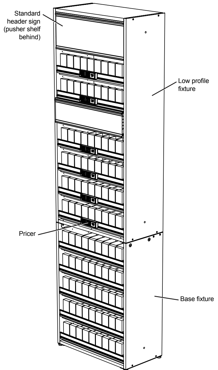
High Profile Fixture
